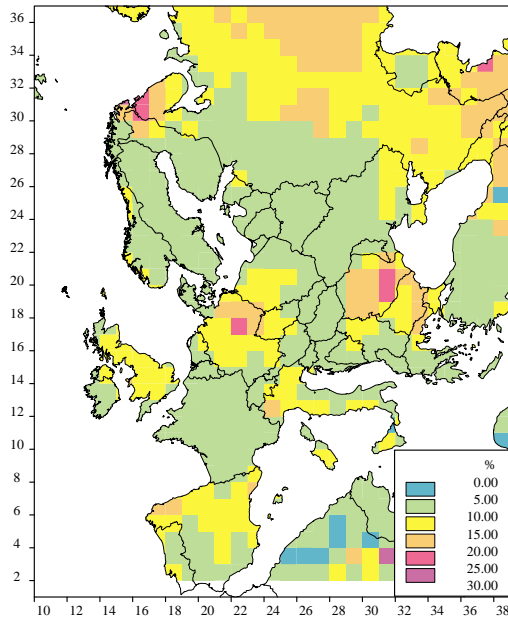
Sulfur deposition
