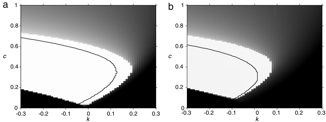
Fig. A.1. Evolution of assortative mating in the single-locus model with mating costs, assuming a single large mutational step. The number of mating trials per female is T = 10 in (a) and T = 5 in (b). Shades of gray indicate the equilibrium frequency (black: 0, white: 1) of an “isolation allele” with m = 1^- = 0.99 introduced at the low frequency p = 10^{-4} into a randomly mating resident population with m_r = 0 . The continuous lines show the corresponding boundaries of the complete-isolation regime for infinitesimally small steps (calculated as in Kopp and Hermisson, 2008).
