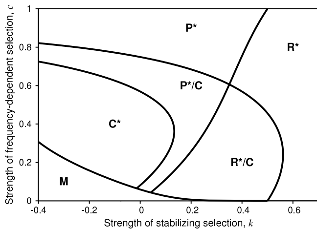
Fig. 1. Evolutionary regimes in the baseline model. The ecological trait is determined by a single locus, and choosiness evolves in infinitesimal steps. Note that negative k implies that selection due to the carrying capacity function is disruptive. C^* : complete isolation; R^* : random mating; P^* : partial isolation; R^*/C : random mating or complete isolation; P^*/C : partial or complete isolation; M : monomorphic outcome with only one extreme phenotype. The asterisk indicates that the outcome is reached from random mating. The boundary for the local stability of random mating and complete isolation is calculated according to Appendix A. The boundary of the C^* regime is calculated numerically using Eq. (11), and the boundary of the M regime is determined by numerical stability analysis as in Pennings et al. (2008).
