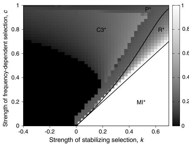
Fig. 5. Frequency of the intermediate phenotype in the two-locus model, when simulations are started from random mating. Shades of gray indicate the frequency of the phenotype x = 0 , ranging from 0 (black) to 1 (white). The upper continuous line shows the border between the R^* and P^* domains, while the lower continuous line shows the border between the R^* and the MI^* domains. Across the R^* domain, the frequency of the intermediate phenotype increases from 0.5 (at the boundary to the P^* domain) to 1 (at the boundary to the MI^* domain). This is achieved by an increasing asymmetry of the allele frequencies at the ecological loci, 0.5 \pm \alpha , with \alpha increasing from 0 to 0.5.
