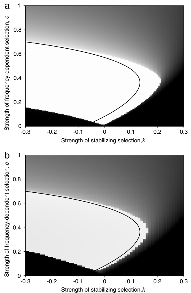
Fig. 2. Evolution of assortative mating in the single-locus model with large mutational steps. (a) Single-step model: An isolation mutant with m = 1^- = 0.99 is introduced at frequency p = 10^{-4} into a resident population with m_r = 0 . (b) Stepwise mutation model with five mating alleles ( m = 0, 0.25, 0.5, 0.75, 0.99 ) and a mutation rate of u = 10^{-6} (see text). Shades of gray indicate the mean choosiness \bar{m} in the population at the end of the simulation (white: \bar{m} = 1^- , black: \bar{m} = 0 ). The continuous line is the boundary of the C^* regime for infinitesimal mutational steps, as in Fig. 1. The white area outside this line shows the additional region where complete isolation is possible via “jumping”. Note that the range of k values shown along the horizontal axis is smaller than in Fig. 1.
