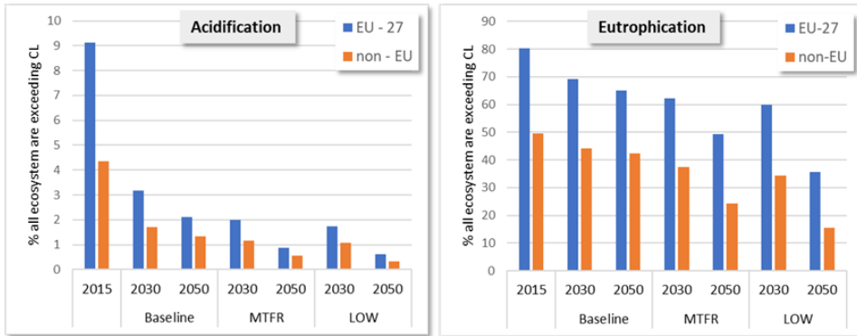
Figure 3: Exceedance of critical loads for acidification and eutrophication in Europe. Non-EU includes West Balkan, UK, Iceland, Norway, Switzerland, Belarus, Ukraine, Moldova, European part of Russia up to 42°E.
