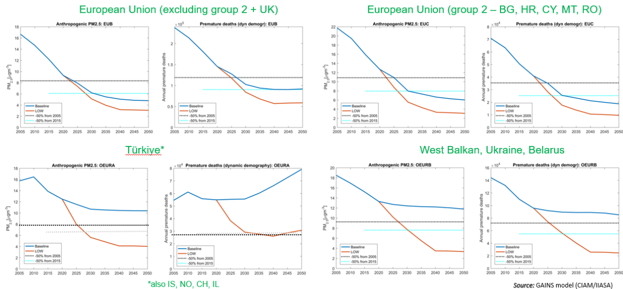
Figure A.1: Change in PM2.5 concentrations and number of premature deaths (taking into account population change and ageing – dynamic demography) for Baseline and LOW scenarios (1) 4
