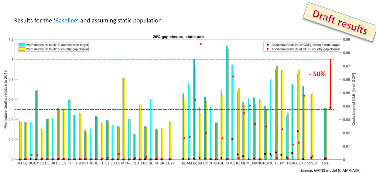
Figure 9: Country outcomes of least cost scenarios for 2050 to reduce premature deaths for the whole UNECE-Europe region by 50% between 2015 and 2050, not considering population changes. Two different variants of target setting are shown (yellow bars/red dots: equal gap closure in each country; cyan bars/black dots: domain wide gap closure without country targets).
