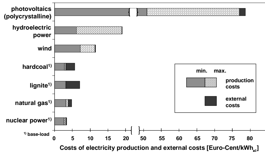
Figure 4: Total costs of various electricity generation technologies operated in Germany
