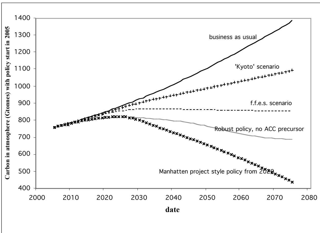
Figure 3: Carbon in atmosphere profiles under various reference scenarios and under robust policy with and without an ACC precursor event in 2020
