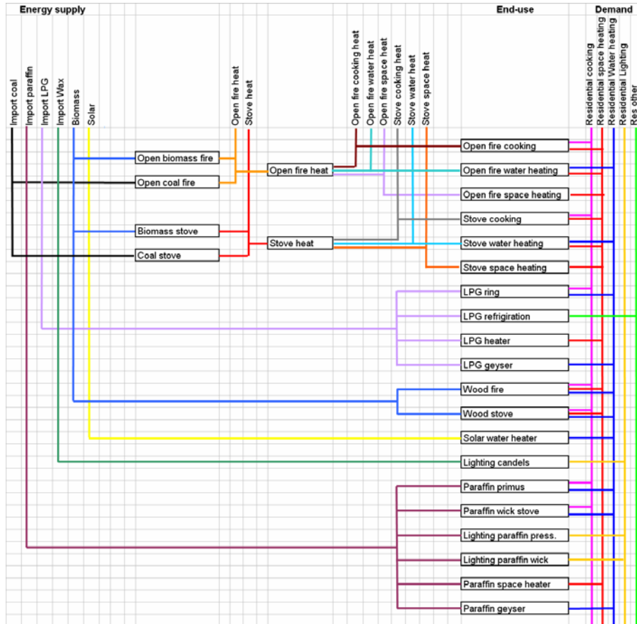
Figure 1: Reference energy system for non-electrified community
